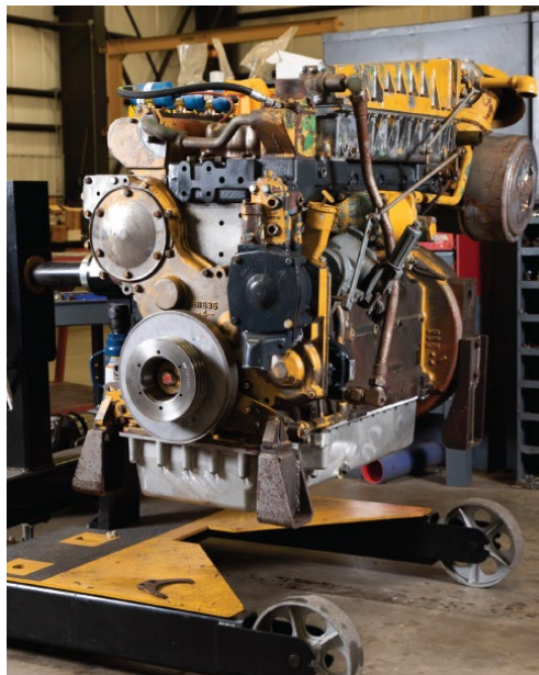
3306TA engine in WPI's Houston Reman Center
